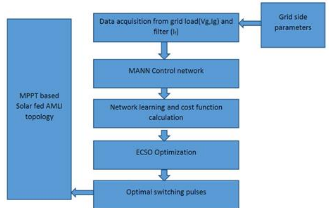
Figure 3. Proposed Controller method
