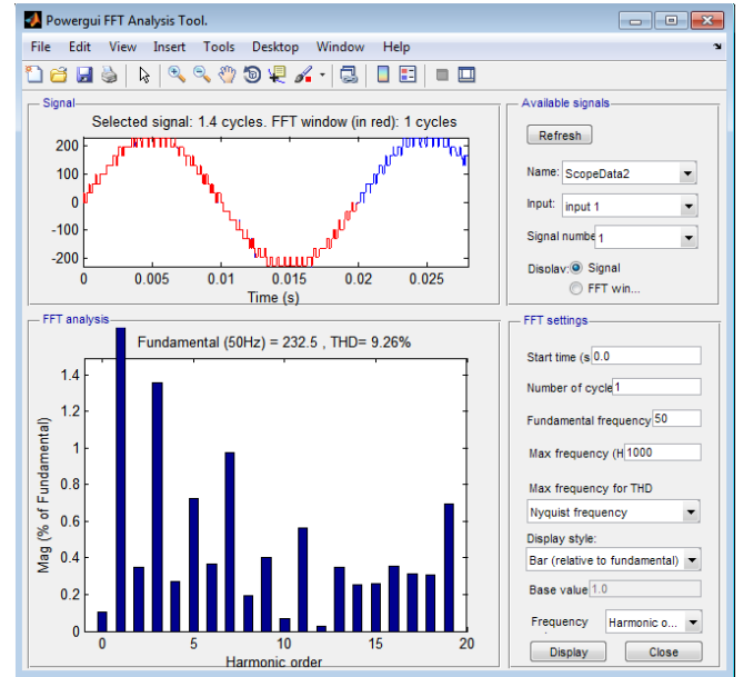
Figure 6. FFT Analysis for 15-level inverter model
