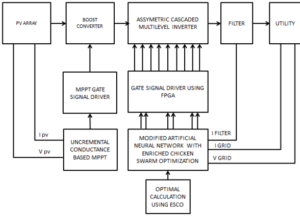
Figure 1. Block diagram of proposed SOLAR FED ASSYMETRIC MLI
