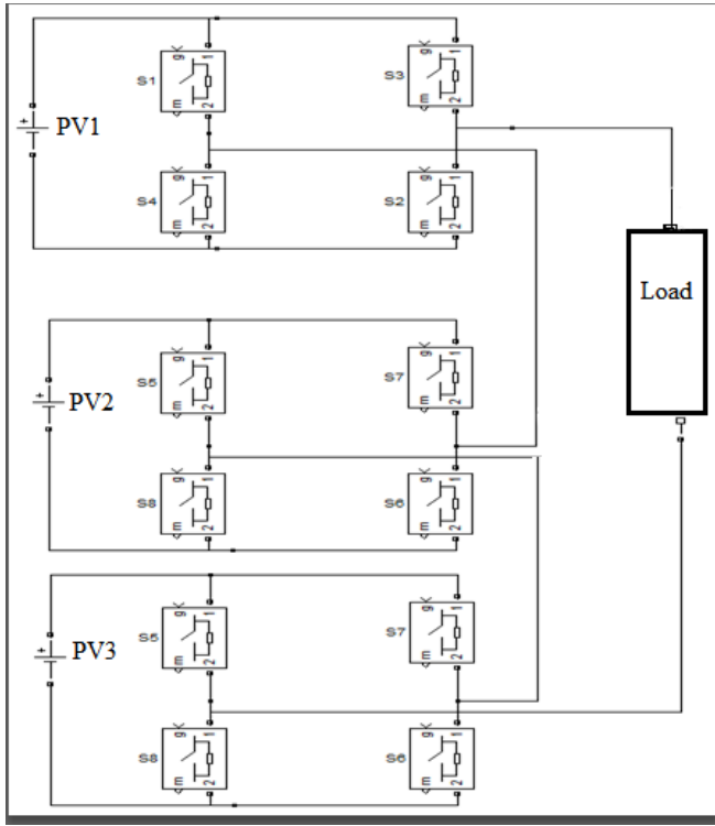
Figure 2. Proposed AMLI Topology
