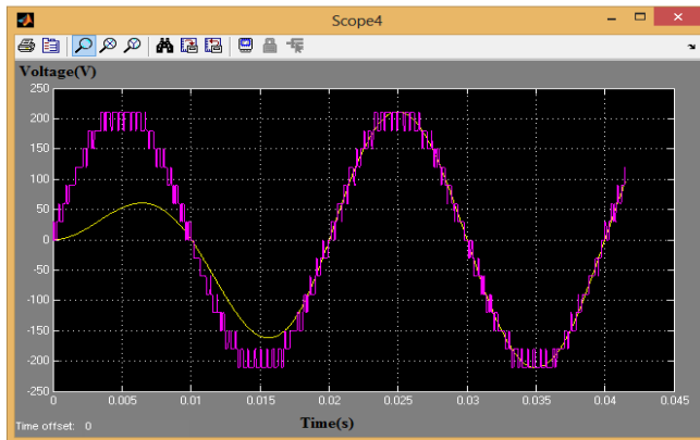
Figure 5. Simulation output voltage for 15-Level MLI using proposed control
