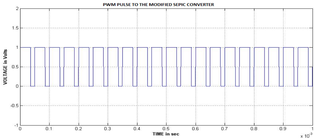
Figure V. PWM pulses to the updated SEPIC converter and inductor current waveform at running condition
