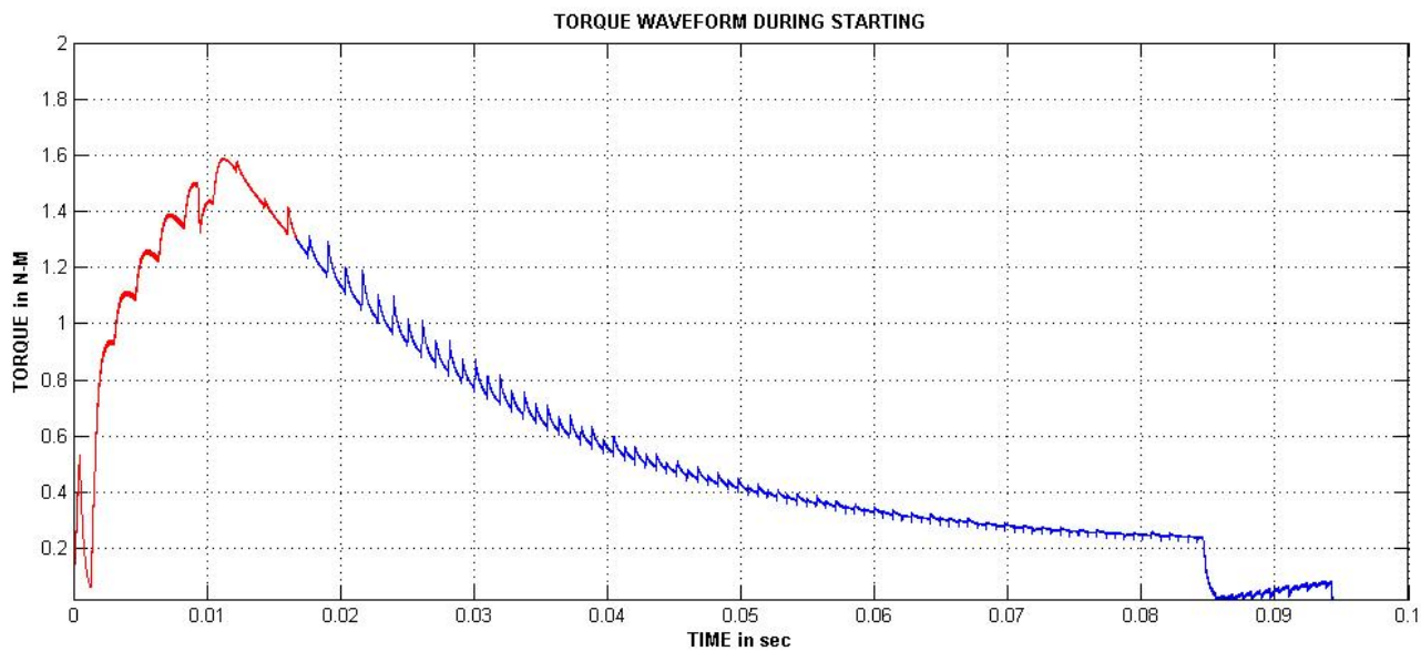
Figure. III. BLDC torque waveform at starting condition
