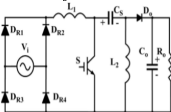
Figure II. Classical SEPIC Converter
