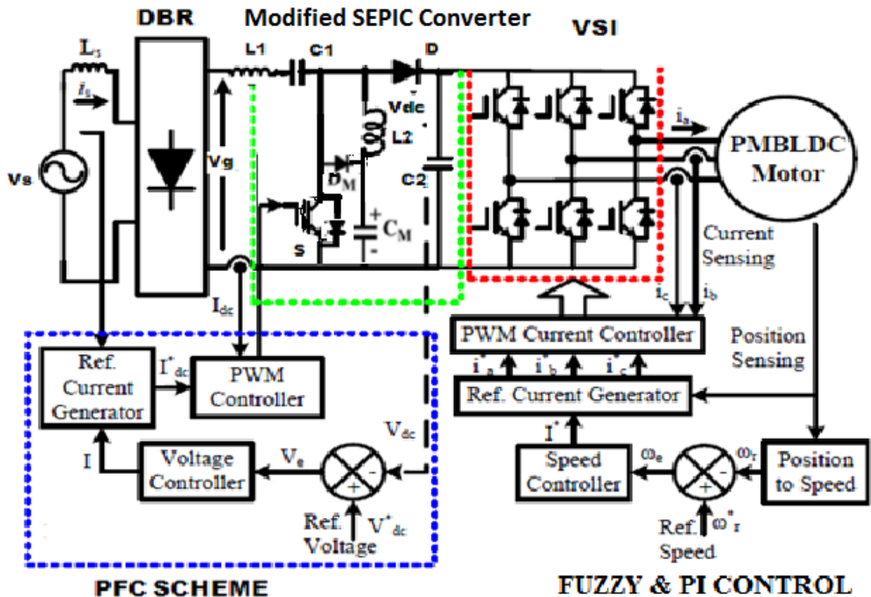
Figure I. Modified PFC SEPIC converter based PMBLDC drive circuit topology
