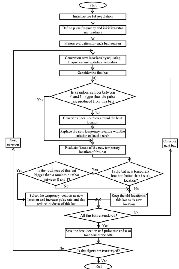
Fig. 4. Flow chart of BAT search algorithm.
