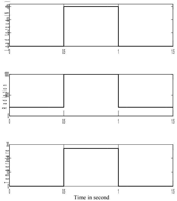
Fig. 15. Step change in load torque and PV system parameters.
