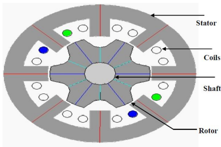
Fig. 2. The SRM 8/6 poles construction.
