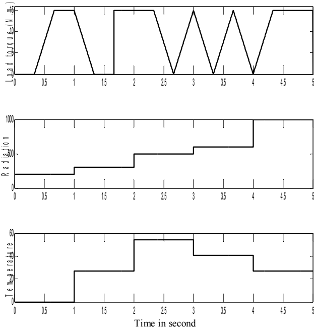
Fig. 18. Change in load torque and PV system parameters.
