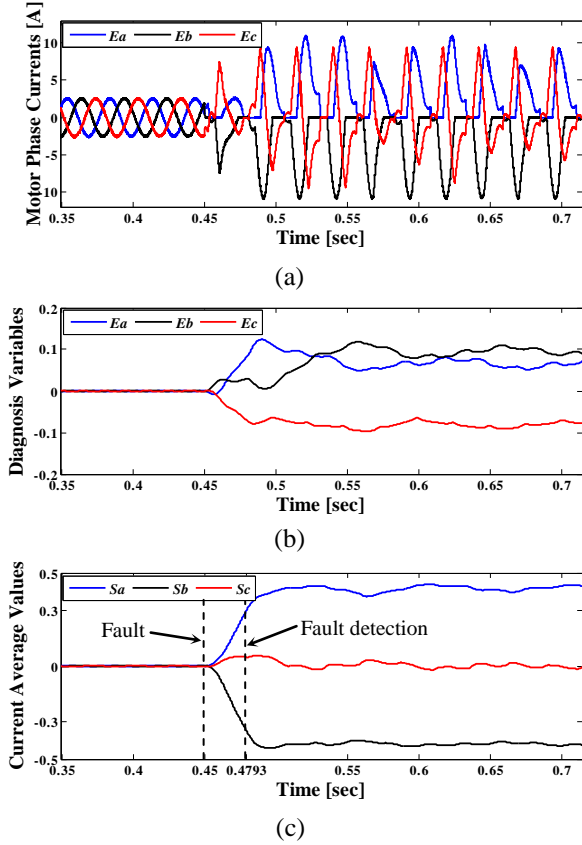
Fig. 8. Simulation results for a crossed double power switch open-circuit fault in IGBTs T2 and T3 of the (a) motor phase currents, (b) diagnosis variables and (c) current average values.
