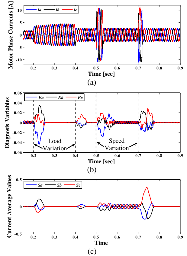
Fig. 9. Simulation results during load and speed variations of the (a) motor phase currents, (b) diagnosis variables and (c) current average values.
