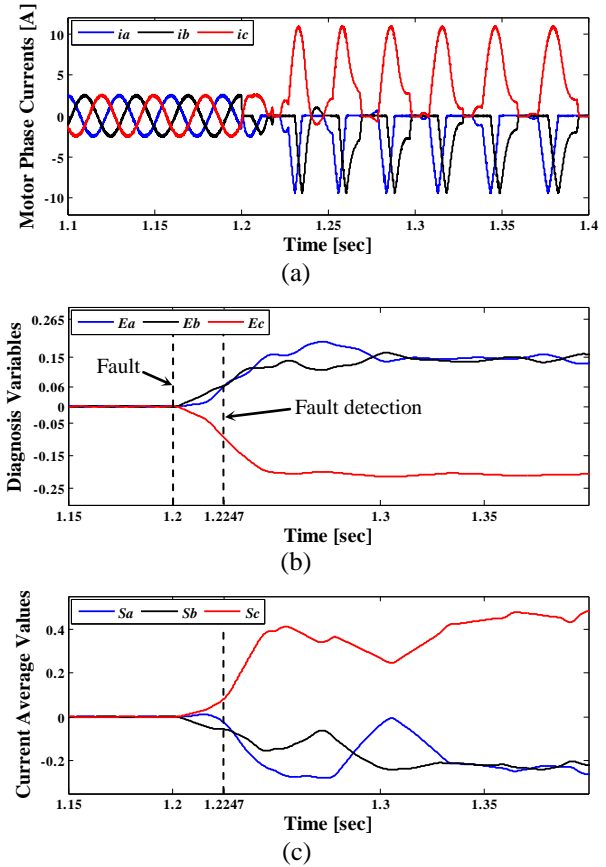
Fig. 7. Simulation results for a double power switch open-circuit fault in IGBTs T1 and T3 of the (a) motor phase currents, (b) diagnosis variables and (c) current average values.
