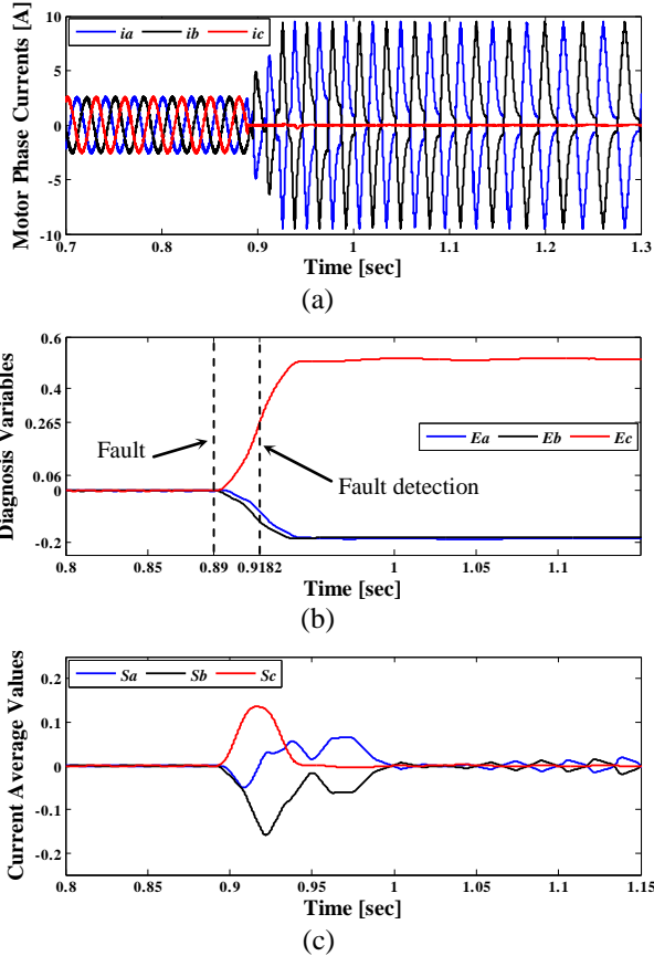
Fig. 6. Simulation results for a single phase open-circuit fault in phase c of the (a) motor phase currents, (b) diagnosis variables and (c) current average values.
