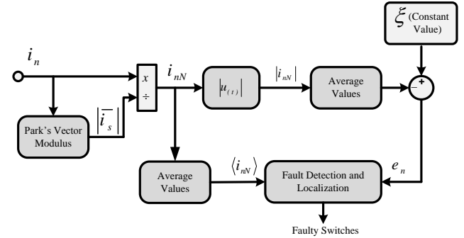
Fig. 1. Block diagram of the fault diagnosis method
