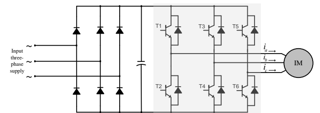
Fig. 2. Diagram of a VSI feeding three-phase induction motor
