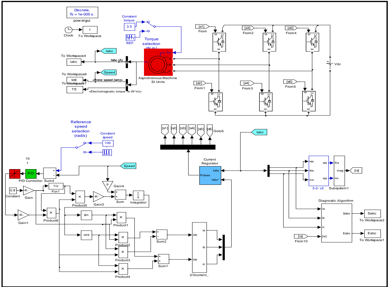
Fig. 4. The MATLAB model of the overall system
