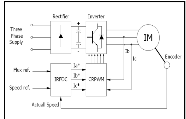
Fig. 3. Block diagram of the field-oriented control strategy
